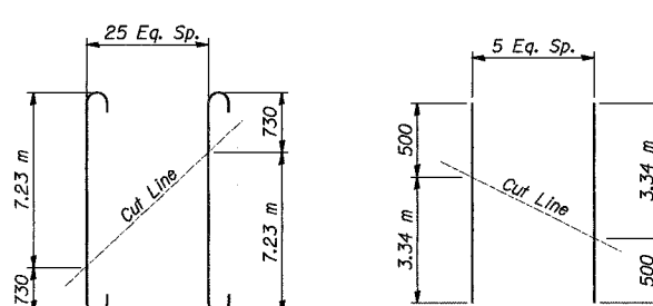
CUTTING DIAGRAM BAR a 10 CUTTING DIAGRAM BAR a 14
