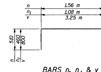
BARS n, n 1 & v
