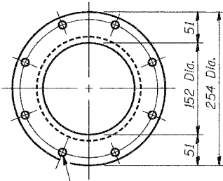
VIEW D-D
