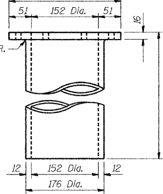
DOWNSPOUT
