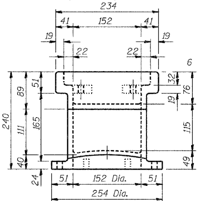
VIEW C-C
