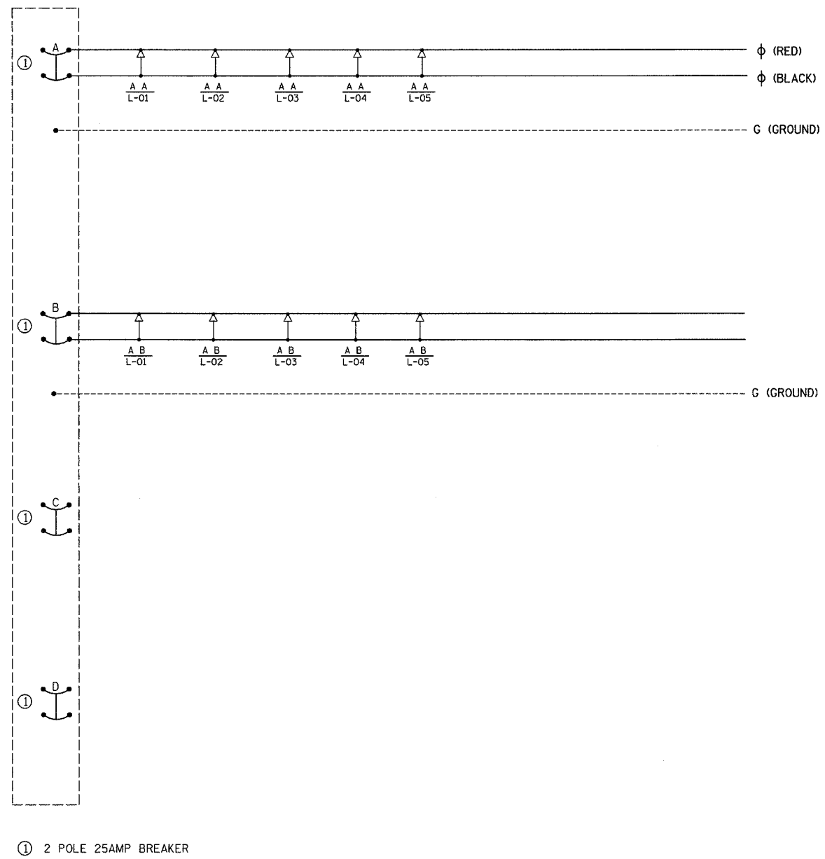
PROPOSED LIGHTING CONTROLLER "A" (1-PHASE, 120/240VOLT, 3-WIRE, 100AMP)
