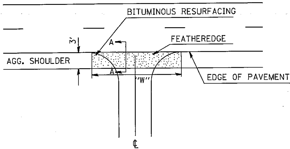
SIDEROAD DETAIL
