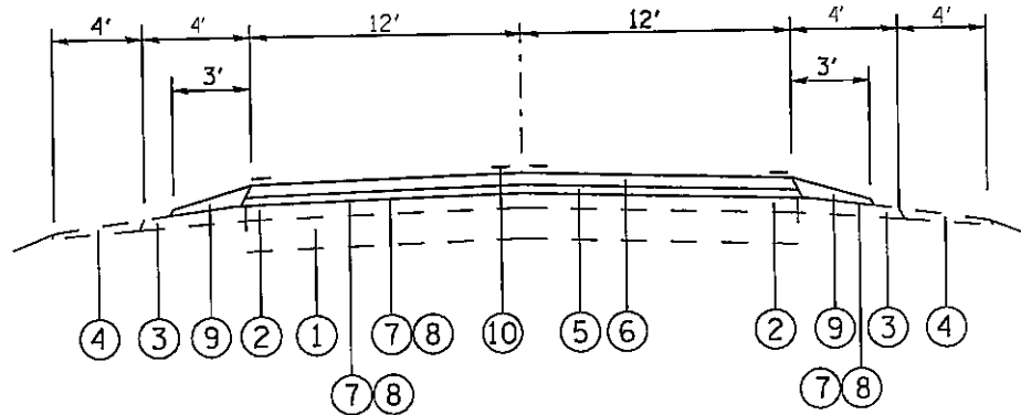
TYPICAL SECTION Mile Pt. 0.486 to Mile Pt. 0.79
