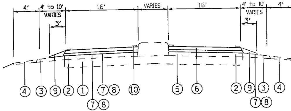
TYPICAL SECTION Mile Pt. 0.00 to Mile Pt. 0.486
