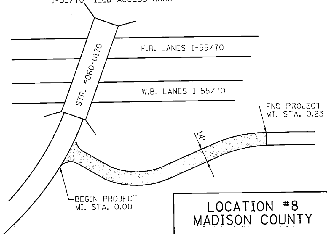
PROJECT LOCATION #8 I-55/70 FIELD ACCESS ROAD
