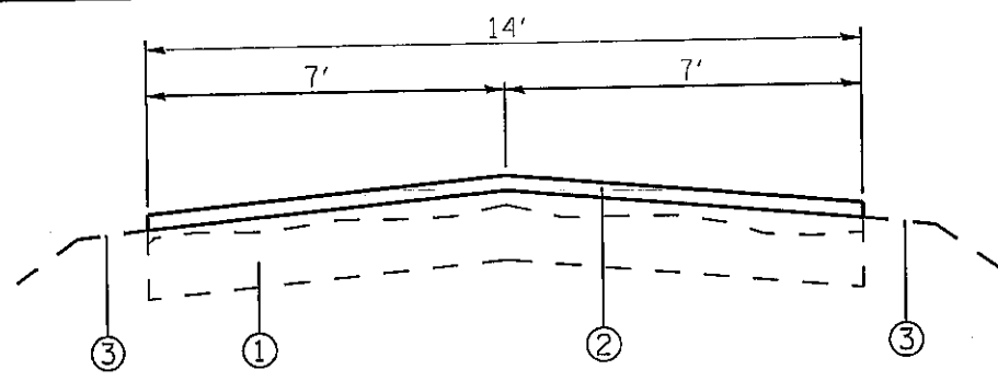
TYPICAL SECTION LOCATION #8
