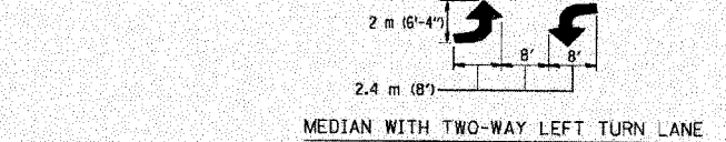
TYPICAL PAINTED MEDIAN MARKING
