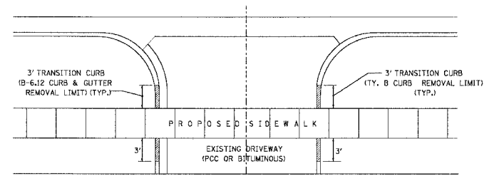
PROPOSED SIDEWALK CROSSING OF DRIVEWAY
