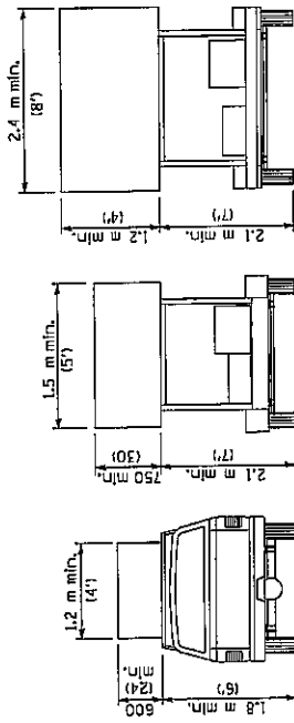
TYPE A ROOF MOUNTED
