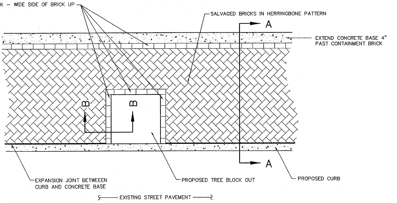
BRICK PAVER SIDEWALK ON CONCRETE BASE (NOT TO SCALE)
