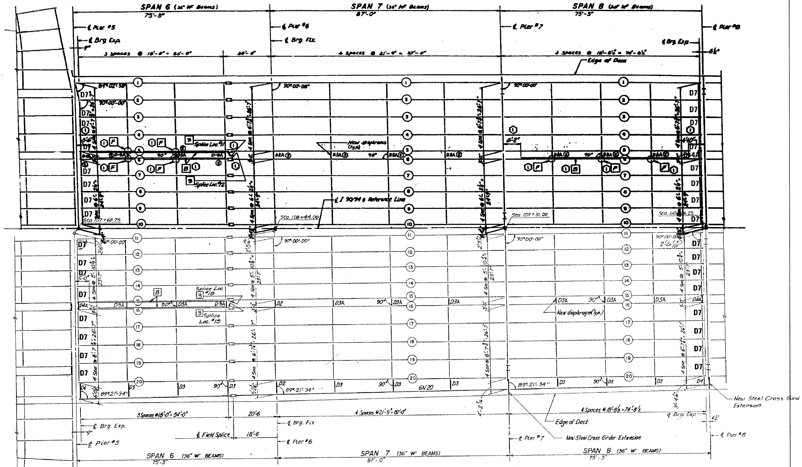
FRAMING PLAN SPANS 6, 7 & 8
