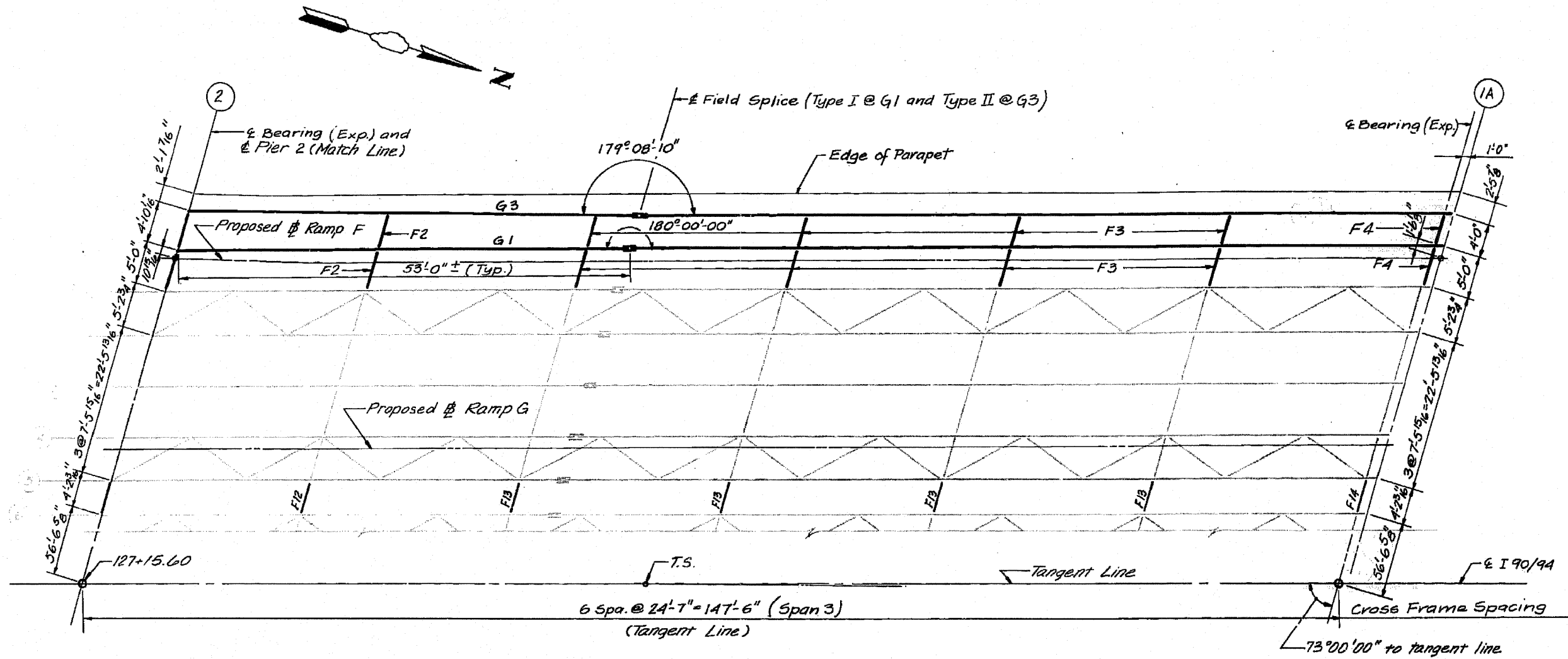
FRAMING PLAN Span 3
