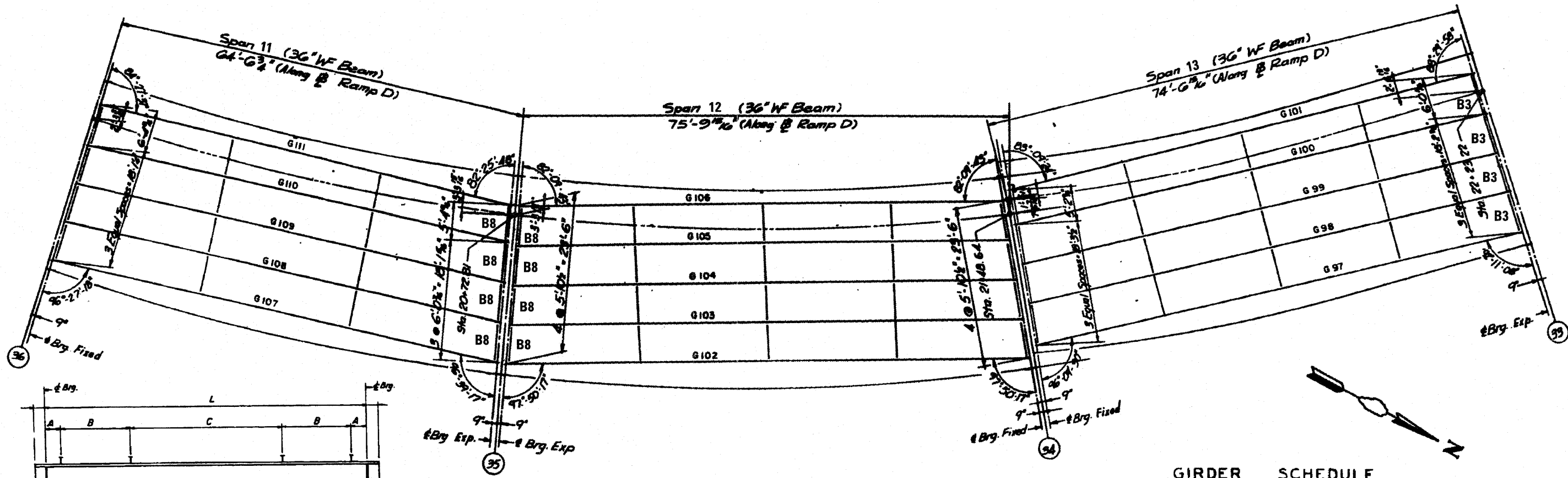
FRAMING PLAN SPANS 11, 12 & 13
