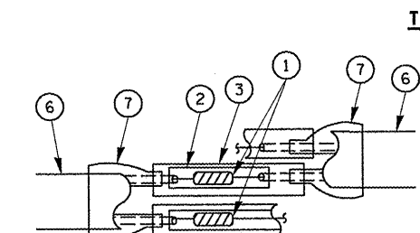
DETAIL "A" LOOP-TO-LOOP SPLICE
