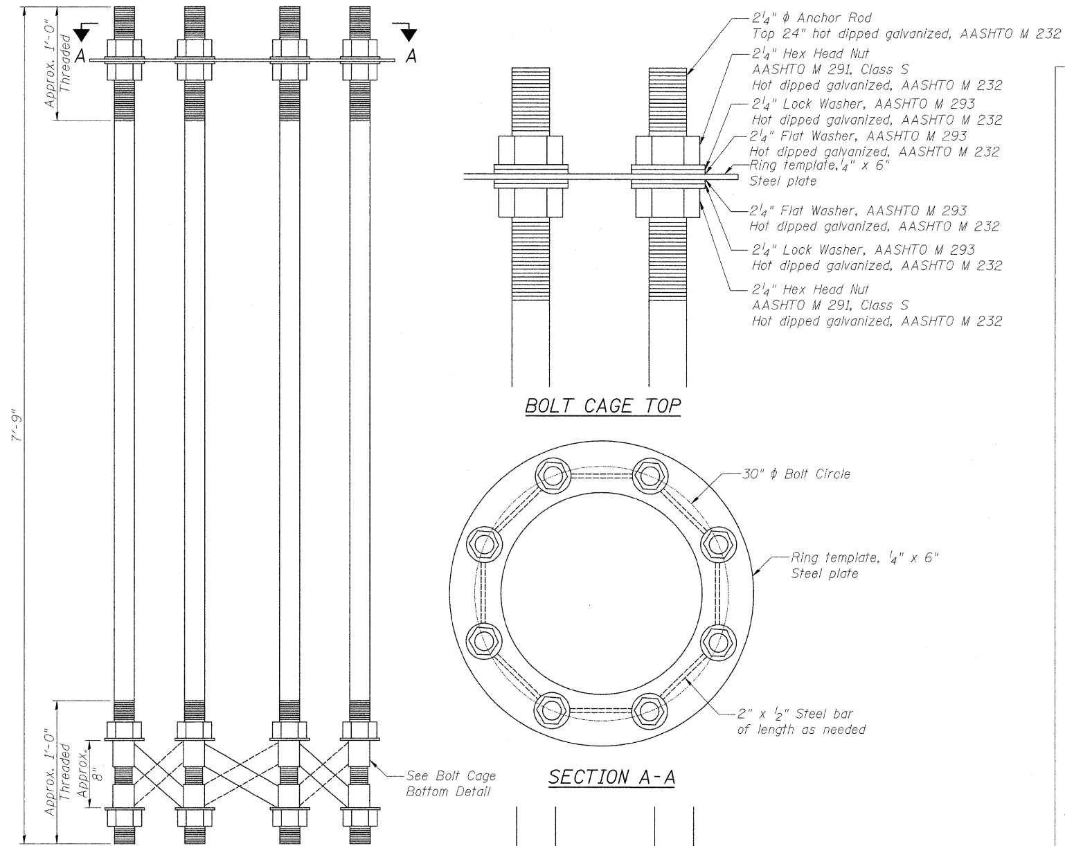
ANCHOR BOLT CAGE
