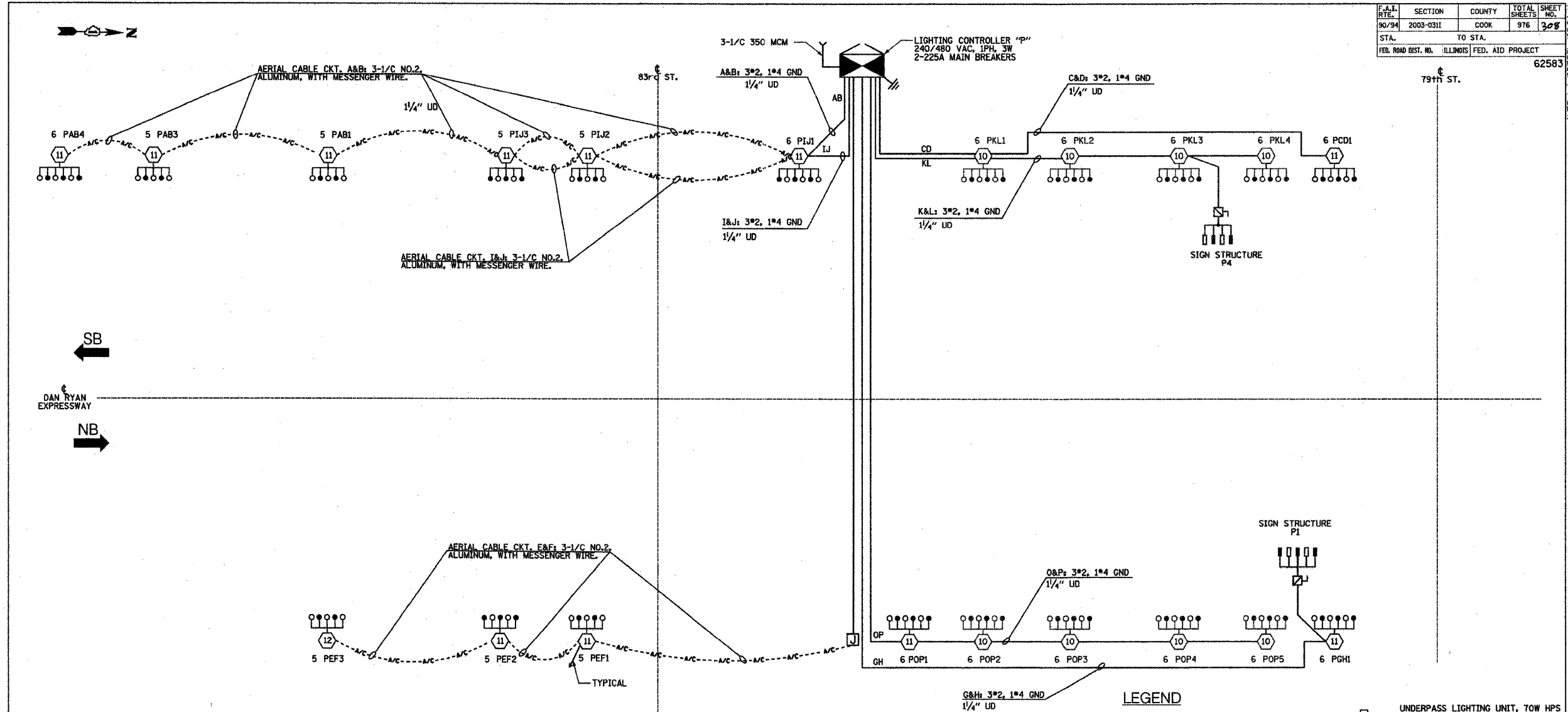
SINGLE LINE DIAGRAM LIGHTING CONTROLLER "P" (NOT TO SCALE)
