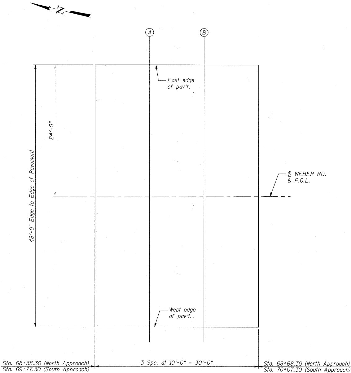
PLAN - APPROACH PAVEMENT
