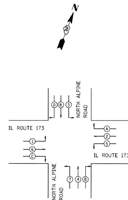
PHASE DESIGNATION DIAGRAM
