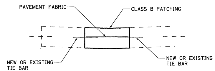
PATCHING DETAIL
