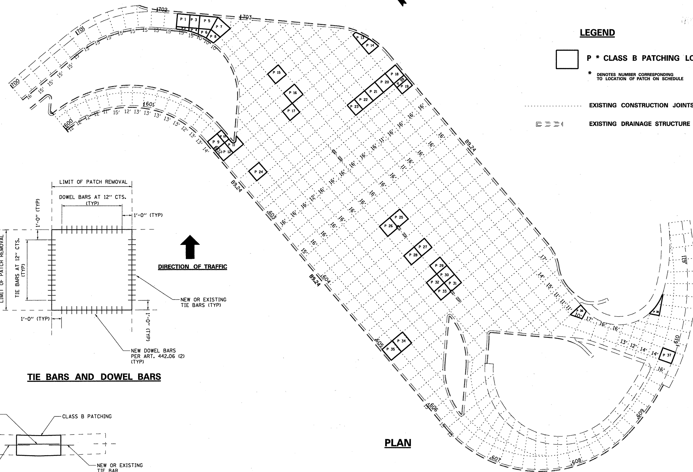
PATCHING DETAIL
