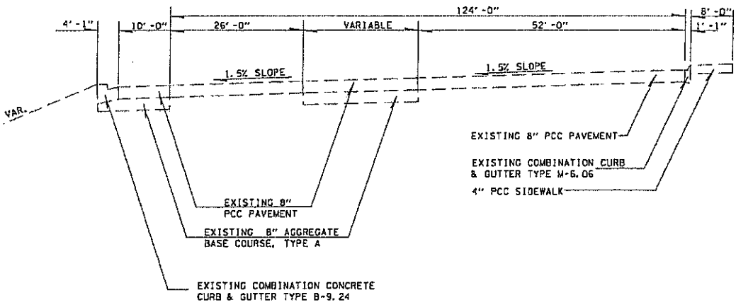
PROPOSED ROADWAY TYPICAL SECTION I-57 @ GREEN CREEK REST AREA- NORTHBOUND
