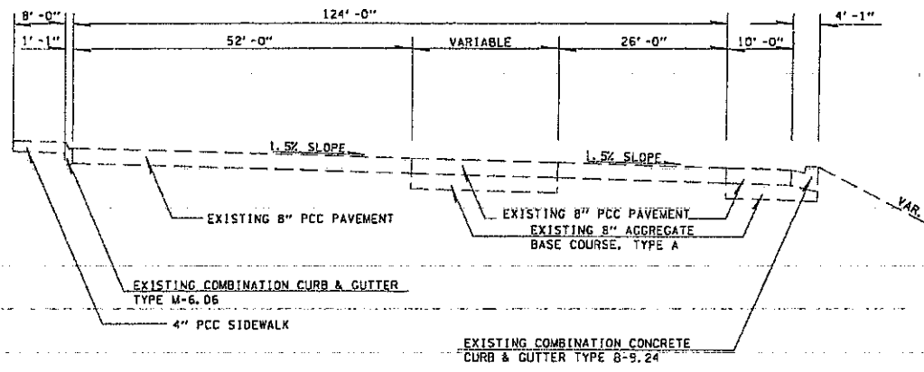
PROPOSED ROADWAY TYPICAL SECTION I-57 @ GREEN CREEK REST AREA- SOUTHBOUND
