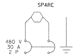
CONTROLLER 2 CIRCUIT 6
