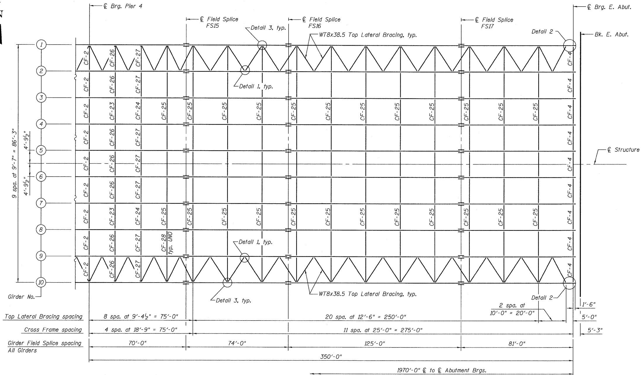
PARTIAL FRAMING PLAN - SPAN 5
