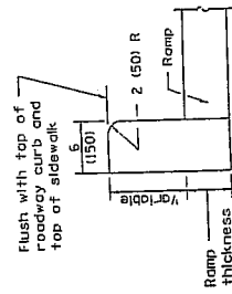
DETAIL OF SIDE CURB
