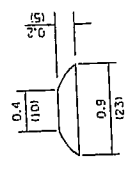
TRUNCATED DOME DETAIL
