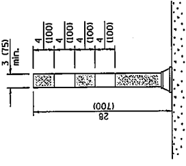
FLEXIBLE DELINEATOR
