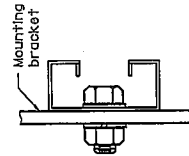
DETAIL C
