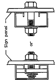
DETAIL A
