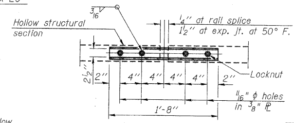
PLAN-BOTT. SPLICE PL TYPICAL
