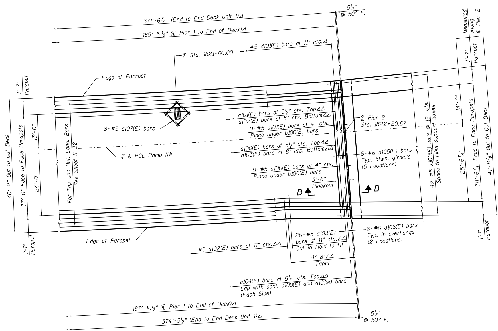
DECK PLAN II - UNIT I
