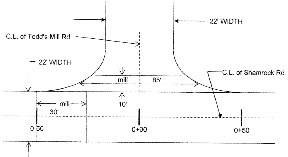
DETAIL OF INTERSECTION WITH TODD'S MILL RD.
