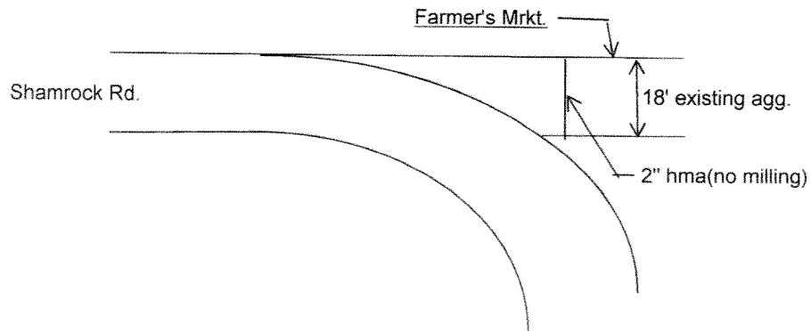
DETAIL OF INTERSECTION WITH FARMER'S MARKET RD.
