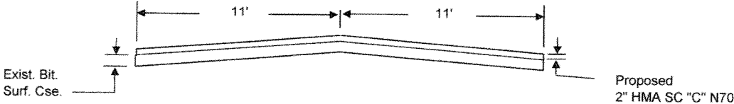
PROPOSED TYPICAL SECTION
