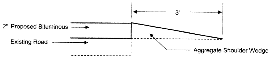
DETAIL FOR AGGREGATE SHOULDER WEDGE
