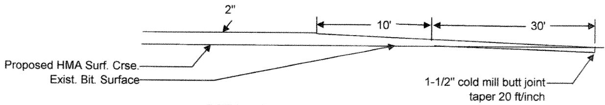
DETAIL OF END TAPERS
