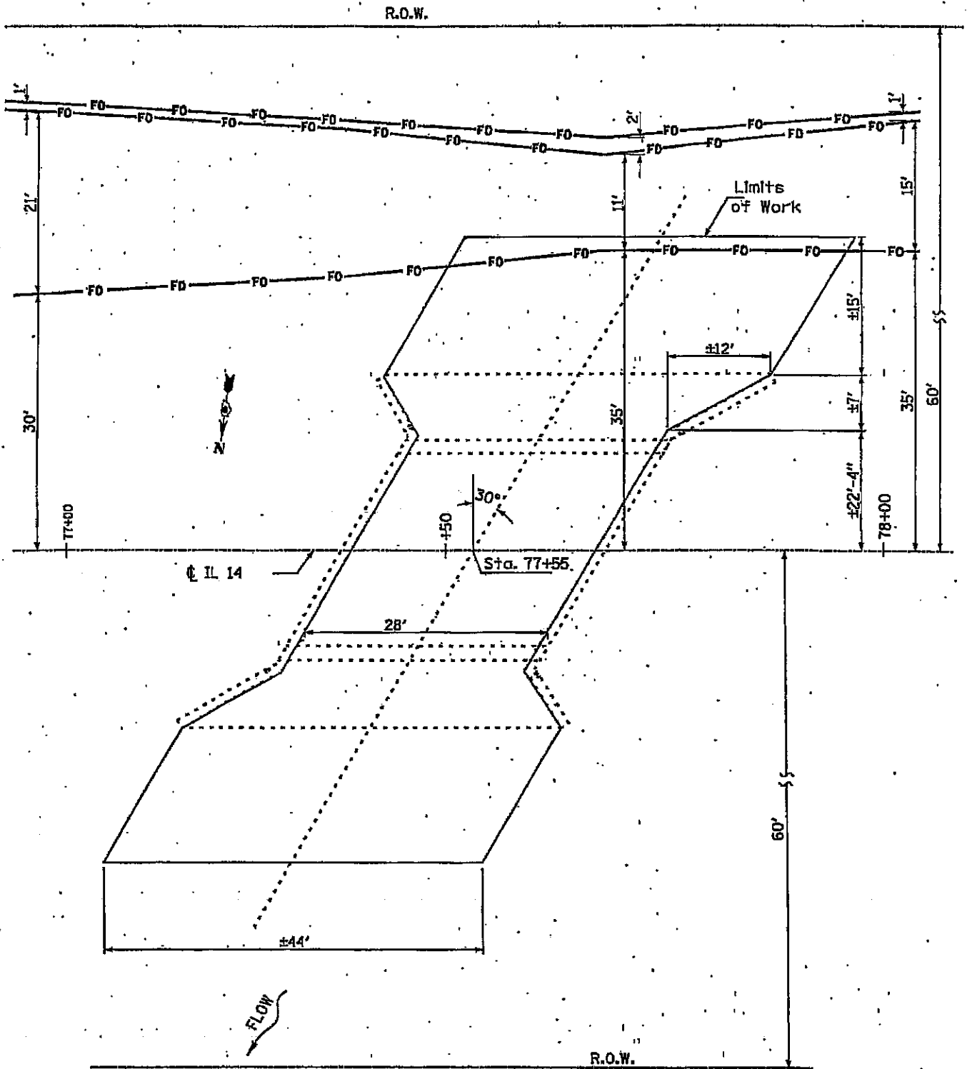
UTILITIES PLAN VIEW 033-0007
