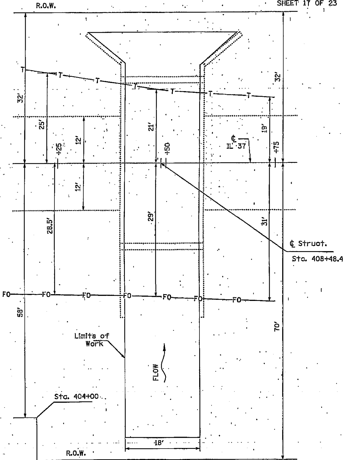
UTILITIES PLAN VIEW 041-0095
