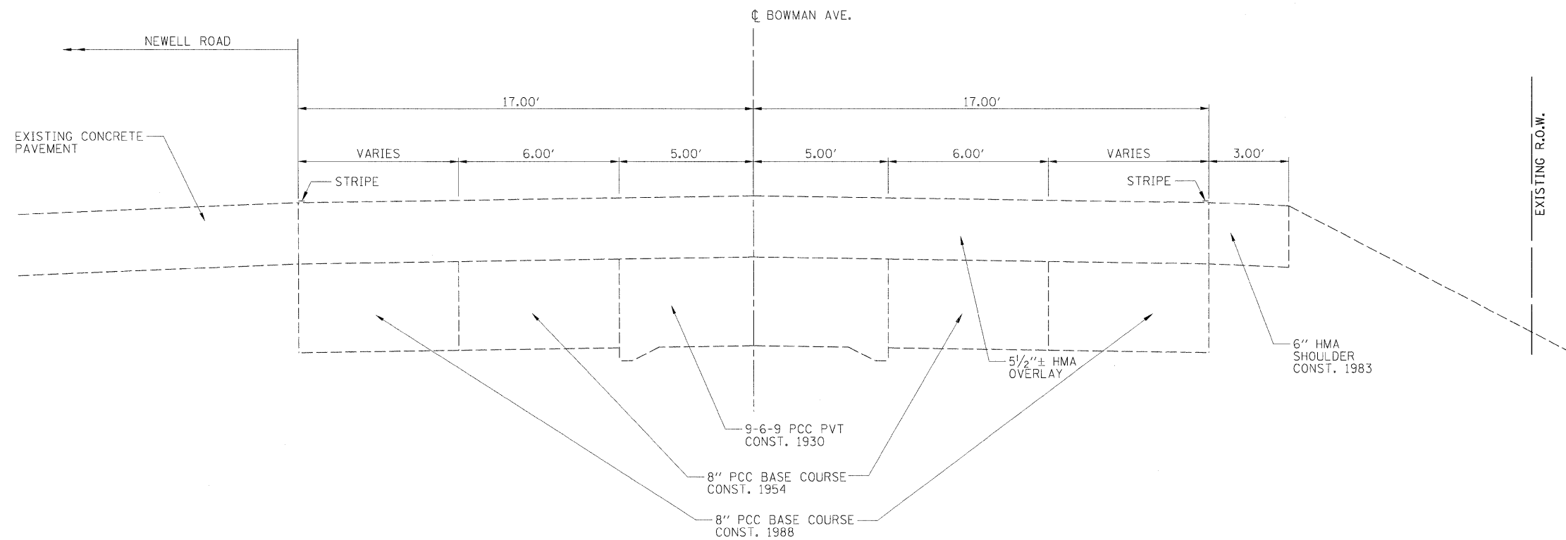
EXISTING TYPICAL SECTION ⑦ STA. 220+90.83 TO STA. 223+30.00
