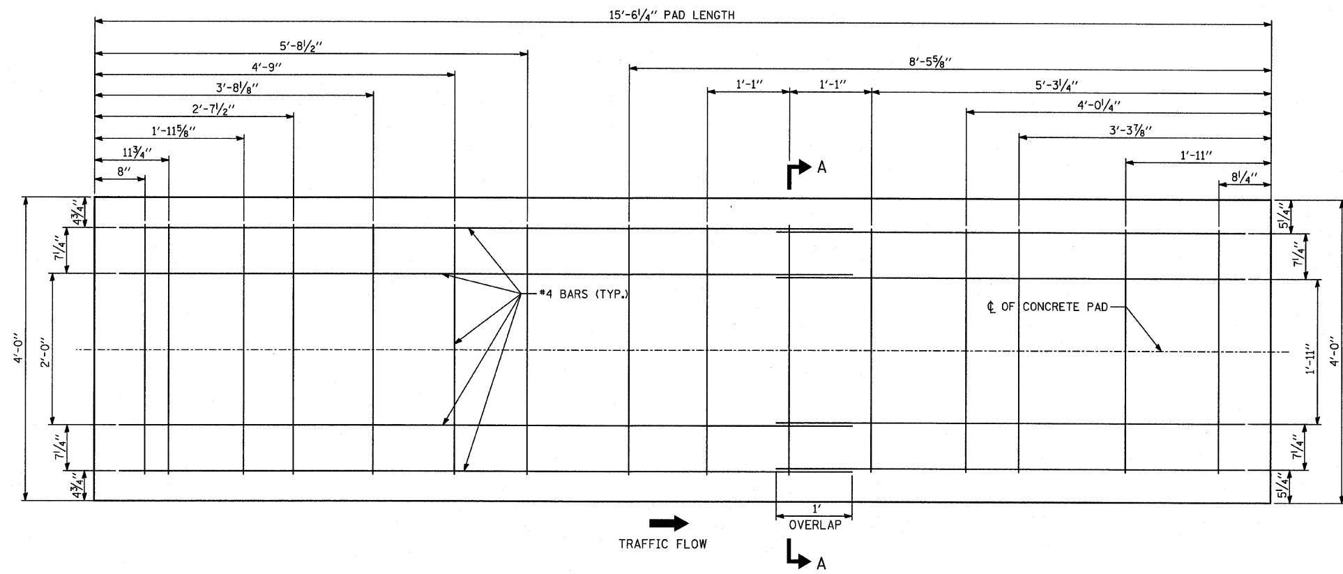
TYPICAL CONCRETE PAD PLAN VIEW
