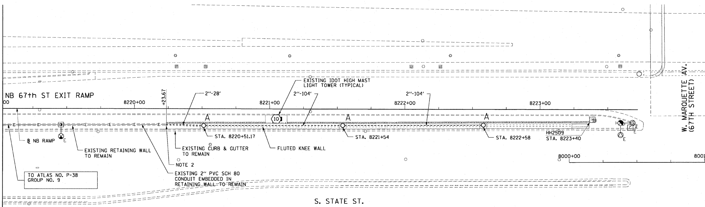
EXISTING CONDUIT/DEMOLITION PLAN
