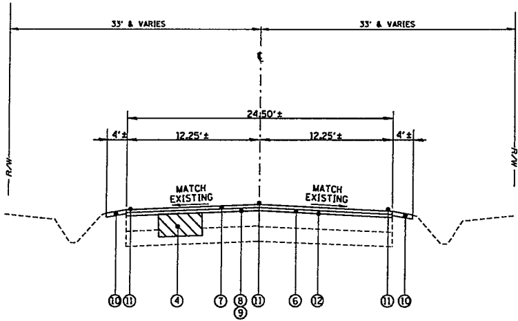
PROPOSED TYPICAL SECTION (RURAL SECTION)
