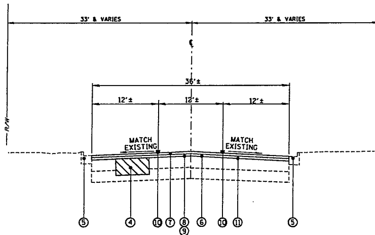
PROPOSED TYPICAL SECTION (URBAN SECTION)
