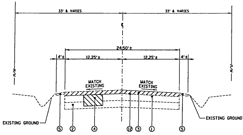
EXISTING TYPICAL SECTION (RURAL SECTION)
