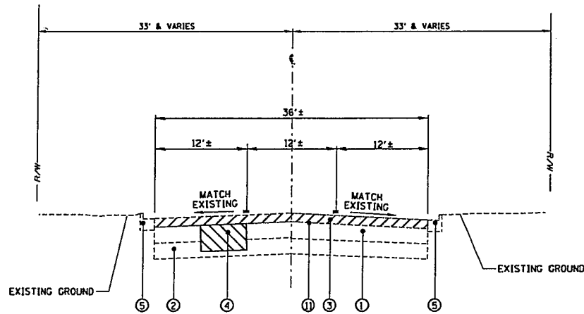
EXISTING TYPICAL SECTION (URBAN SECTION)
