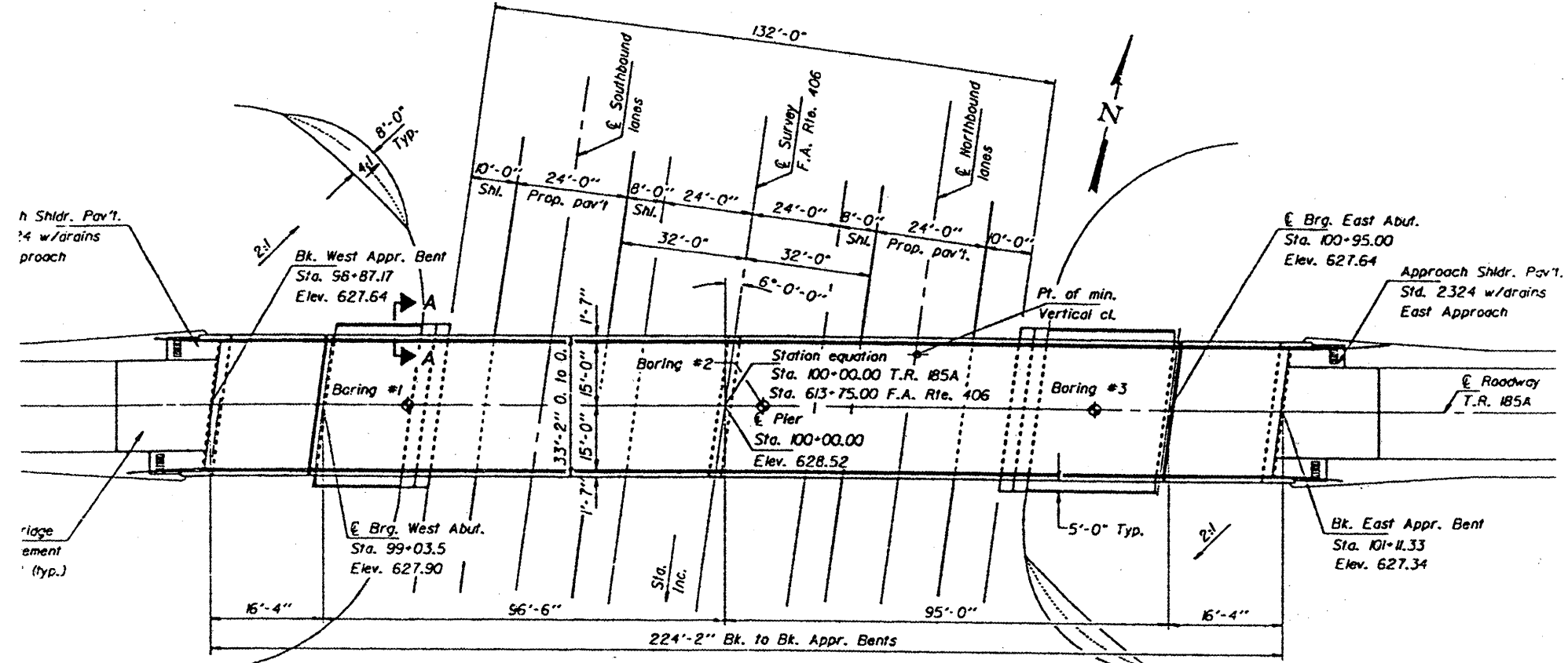
PLAN
