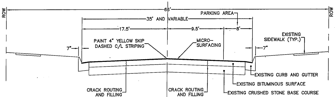
NORTH ST. - OAKWOOD AV. TO CHICAGO ST. STA. 200+00 TO STA. 227+30 SEGMENT "C"
