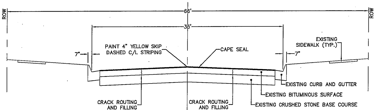
MAIN ST. - OAKWOOD AV. TO CHICAGO ST. STA. 300+00 TO STA. 327+20 SEGMENT "D"
