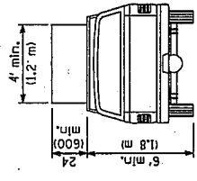
TYPE A ROOF MOUNTED
