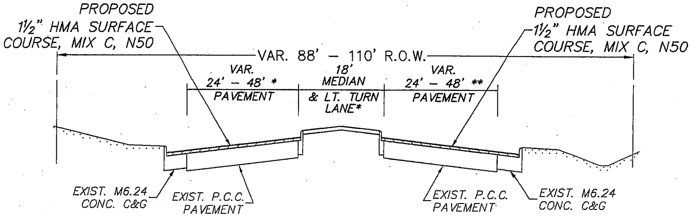
TYPICAL SECTION WINDSOR ROAD
