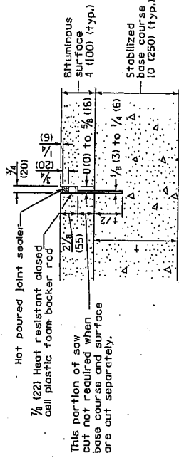
TRANSVERSE CONTRACTION JOINT (FOR CAM, CFA AND LFA BASE COURSE MIXTURES)
