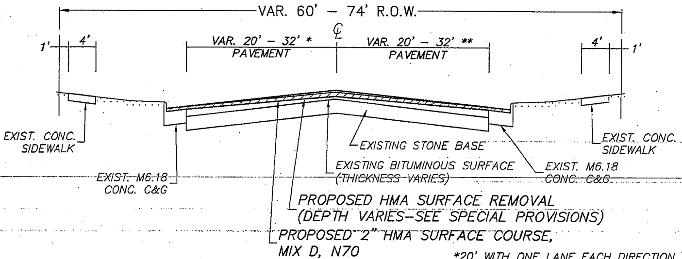
TYPICAL SECTION RIVERSIDE BOULEVARD
