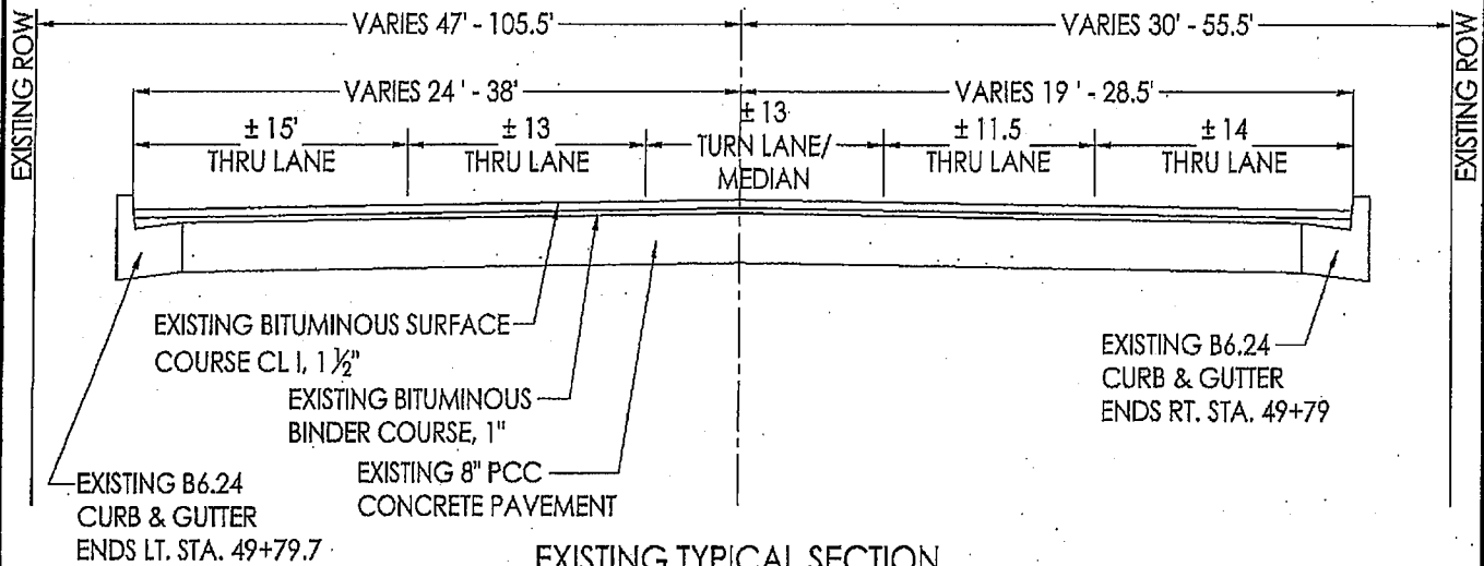
EXISTING TYPICAL SECTION STA. 40+68 TO 51+53 OMISSION STA. 42+87 TO STA. 45+91 (KOCHER ST. TO COMMERCIAL ENTRANCE)
