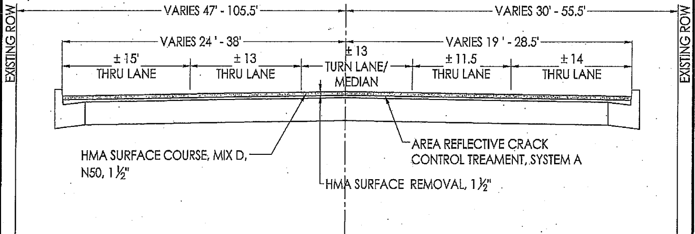
PROPOSED TYPICAL SECTION STA. 40+68 TO 51+53 OMISSION STA. 42+87 TO STA. 45+91 (KOCHER ST. TO COMMERCIAL ENTRANCE)
