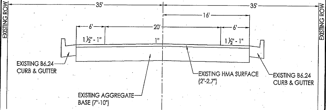
EXISTING TYPICAL SECTION STA. 10+01 TO 28+50 OMISSION STA. 19+48 TO STA. 19+58 (BLACKHAWK BLVD. TO SALEM ST.)
