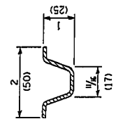
SECTION E-E 1.12 lbs./ft. Steel - (1.67 kg/m)
