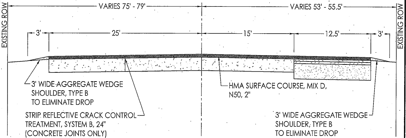
TYPICAL PROPOSED SECTION STA. 51+53 TO 53+40 (THRU COMMERCIAL ENTRANCE)
