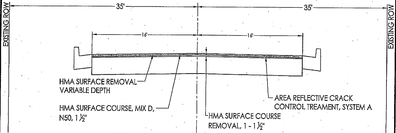
PROPOSED TYPICAL SECTION STA. 10+01 TO 28+50 OMISSION STA. 19+48 TO STA. 19+58 (BLACKHAWK BLVD. TO SALEM ST.)
