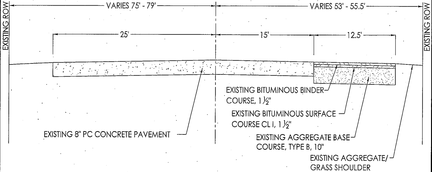
TYPICAL EXISTING SECTION STA. 51+53 TO 53+40 (THRU COMMERCIAL ENTRANCE)
