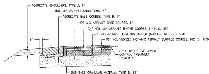
INSERT B NOT TO SCALE
