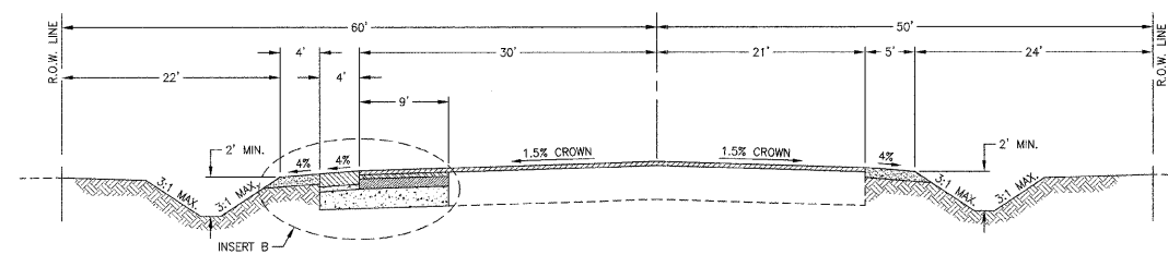
US ROUTE 45/52 - STA. 200+00 TO STA. 203+74 NOT TO SCALE
