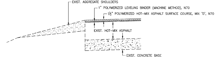
INSERT C NOT TO SCALE
