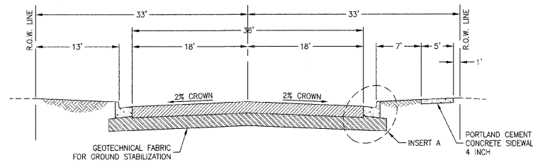
BURNS ROAD EAST - STA. 53+33.50 TO STA. 55+90 NOT TO SCALE
