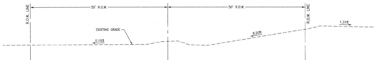
BURNS ROAD WEST - STA. 33+67 TO STA. 53+33.50 NOT TO SCALE
