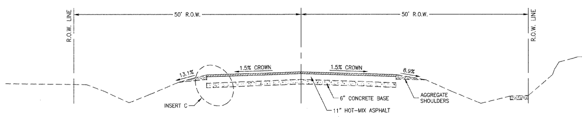
US ROUTE 45/52 - STA. 193+64 TO STA. 200+00 NOT TO SCALE
