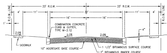
EXISTING SIDE STREETS TYPICAL PAVEMENT SECTION NOT TO SCALE
