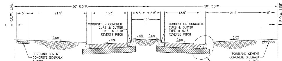
BURNS ROAD WEST - STA. 33+67 TO STA. 53+33.50 NOT TO SCALE
