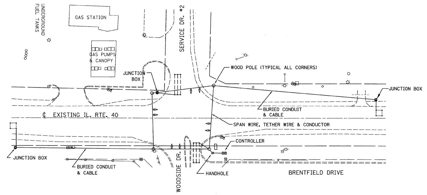
STAGE I EXISTING TRAFFIC SIGNAL
