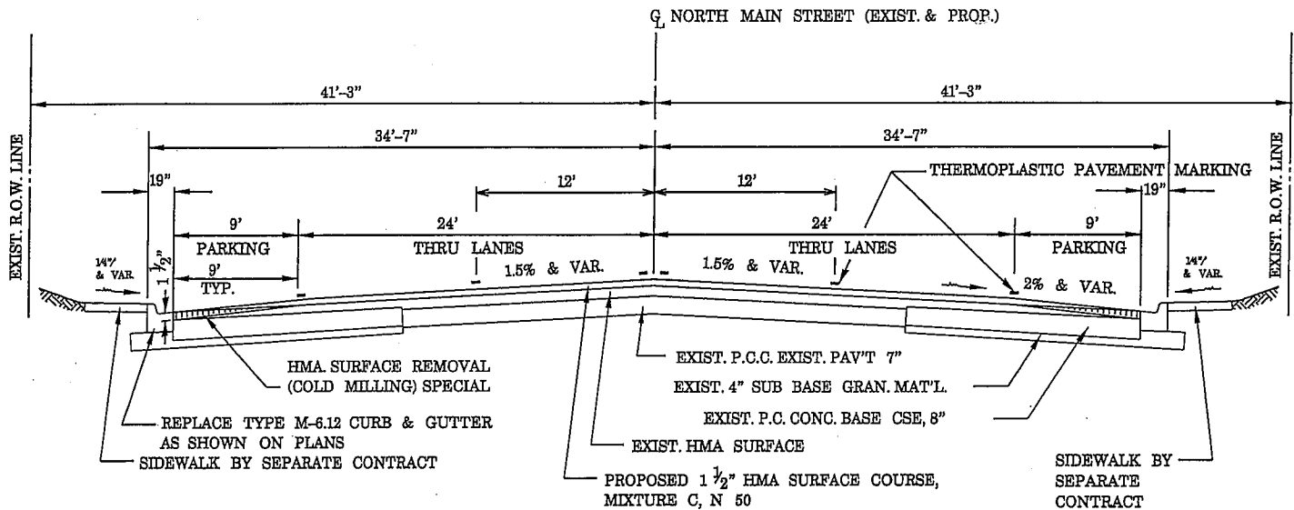
TYPICAL SECTION SECTION 09-00073-00-RS STATION 32+24 - 42+70 STATION 54+03 - 63+77 CITY OF MONMOUTH
