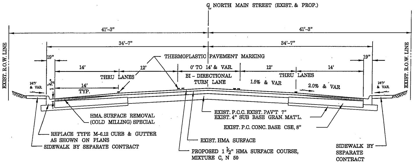
TYPICAL SECTION SECTION 09-00073-00-RS STATION 42+70 - 54+03 CITY OF MONMOUTH
