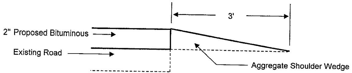
DETAIL FOR AGGREGATE SHOULDER WEDGE
