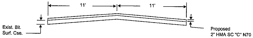
PROPOSED TYPICAL SECTION
