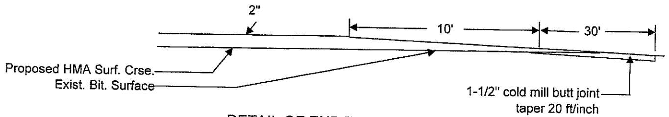
DETAIL OF END TAPERS
