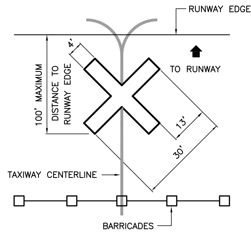
CLOSED TAXIWAY MARKER DETAIL NOT TO SCALE
