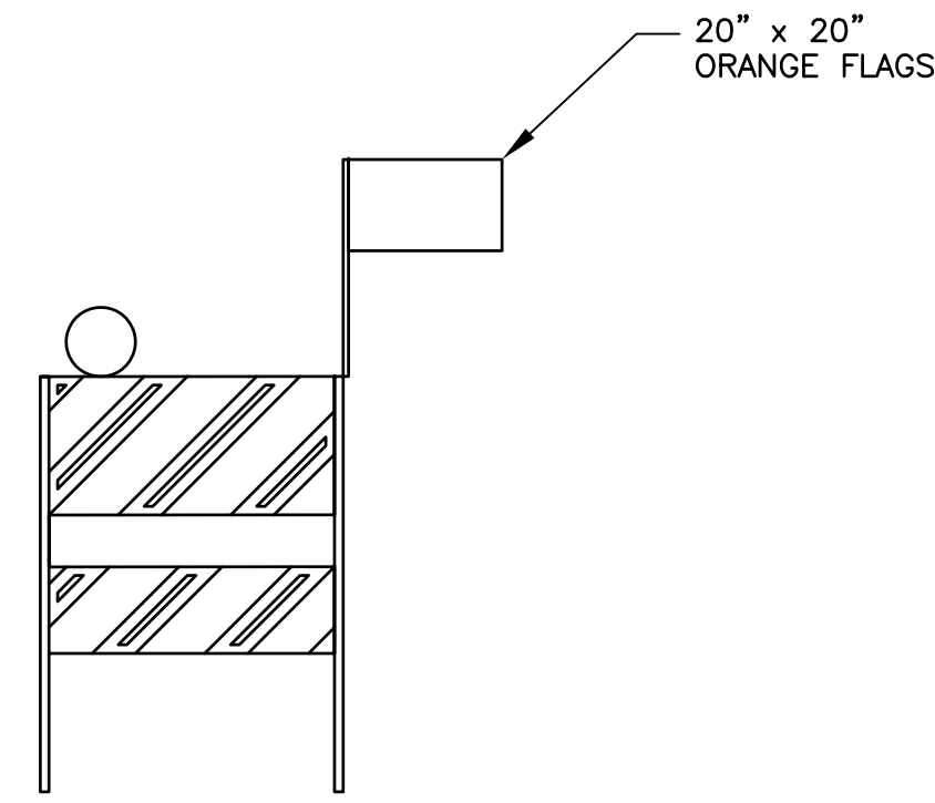
FLASHER BARRICADE DETAIL-IDOT TYPE 2 NOT TO SCALE
