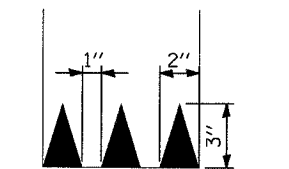
CUT NOTCHES IN INSPECTION PIPE
