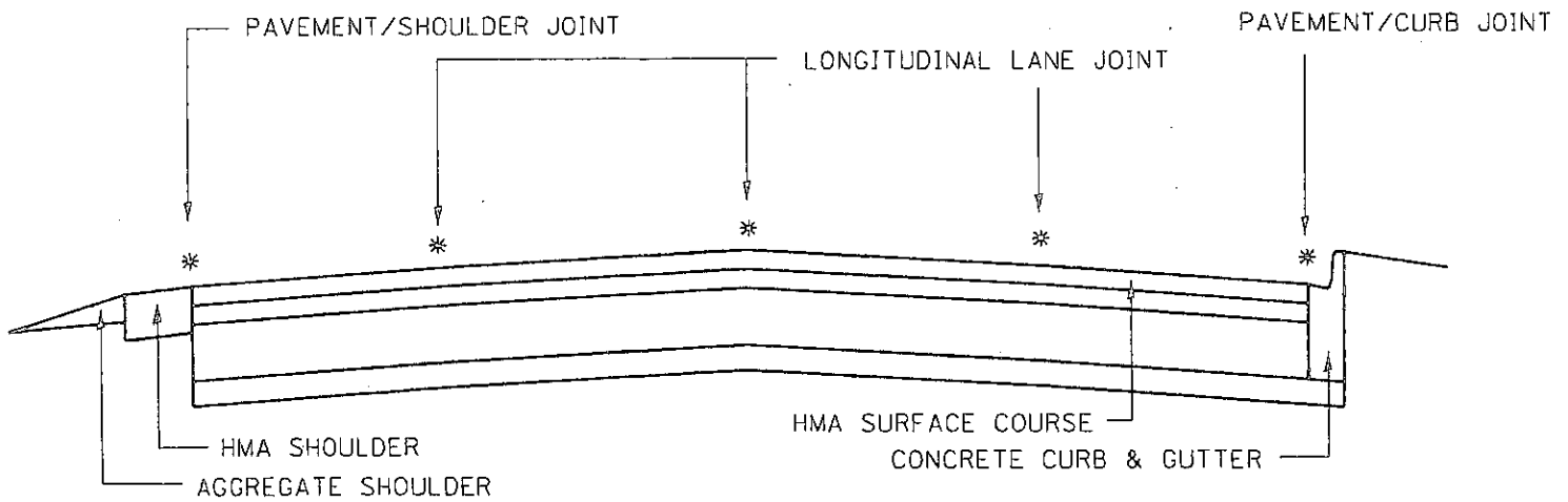
MULTI-LANE UNDIVIDED PAVEMENT
