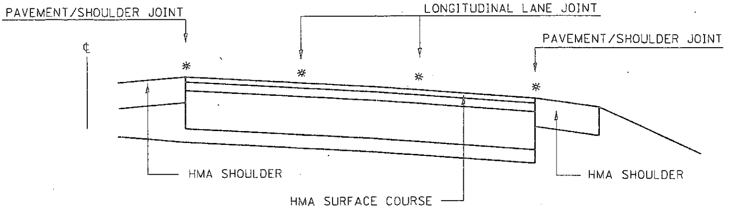
MULTI-LANE DIVIDED PAVEMENT
