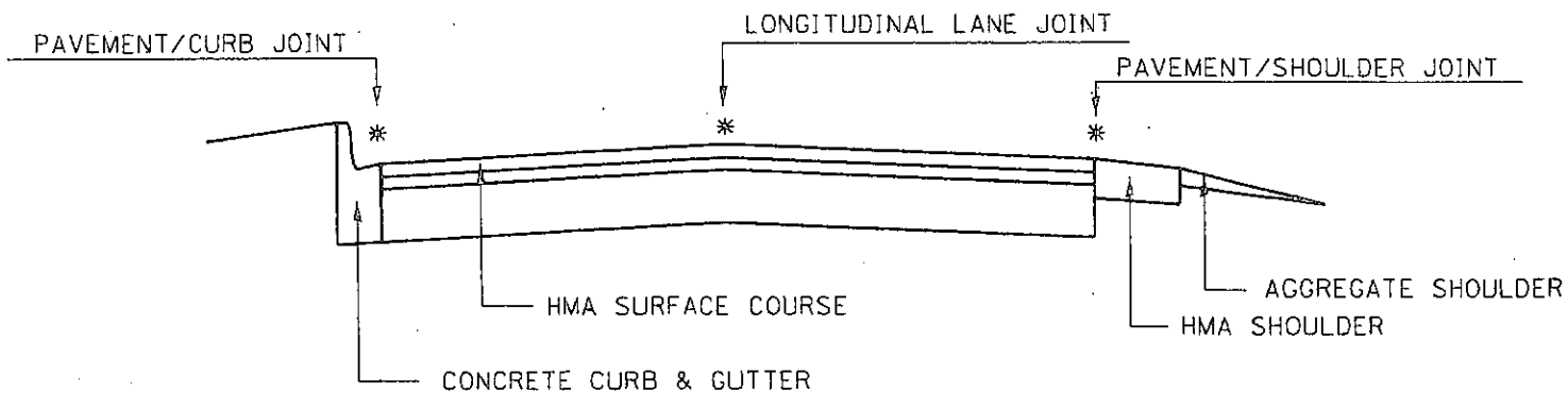
TWO-LANE PAVEMENT
