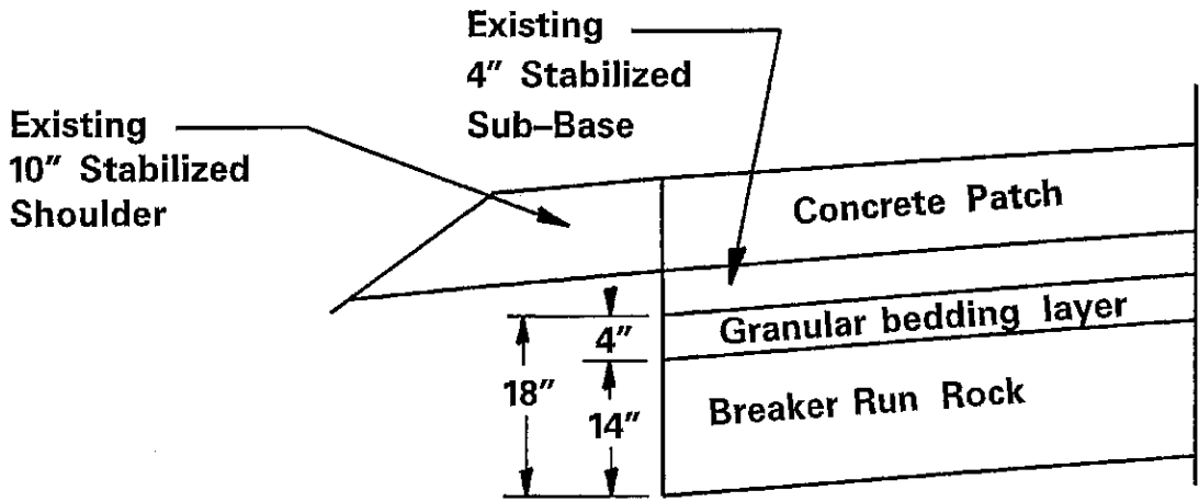
Granular SubGrade Replacement 18 Inch Detail (See Schedule for locations where this is required)
