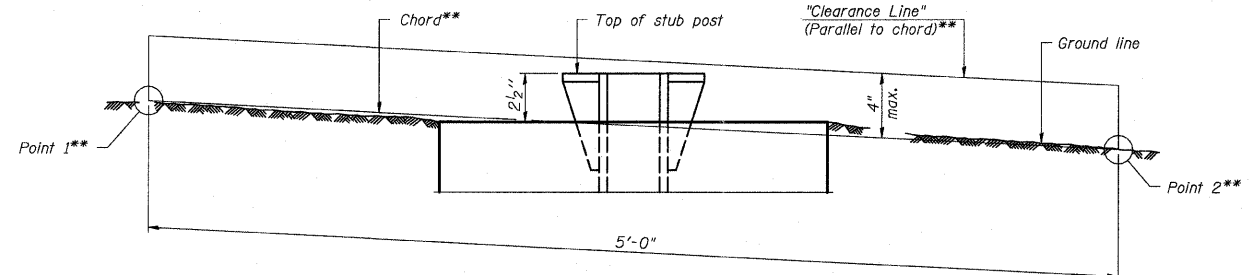
ELEVATION GROUND LINE & STUB POST
