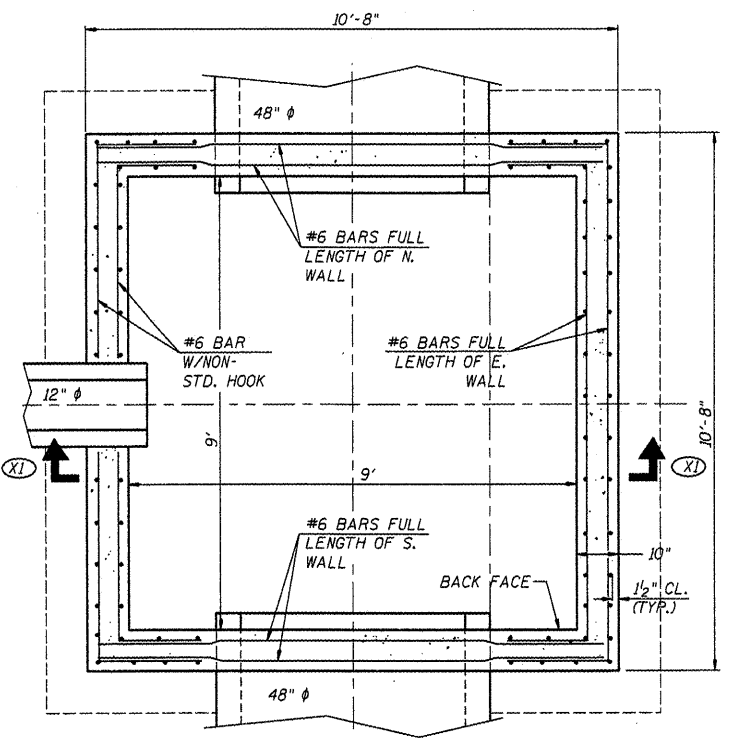
PLAN - TOP PORTION OF BOX
