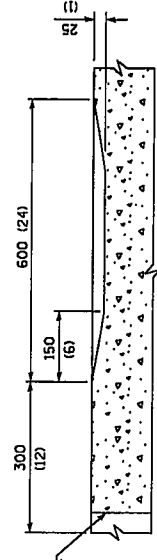
SECTION C-C
