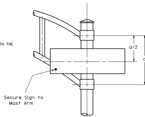
DUAL ARM
