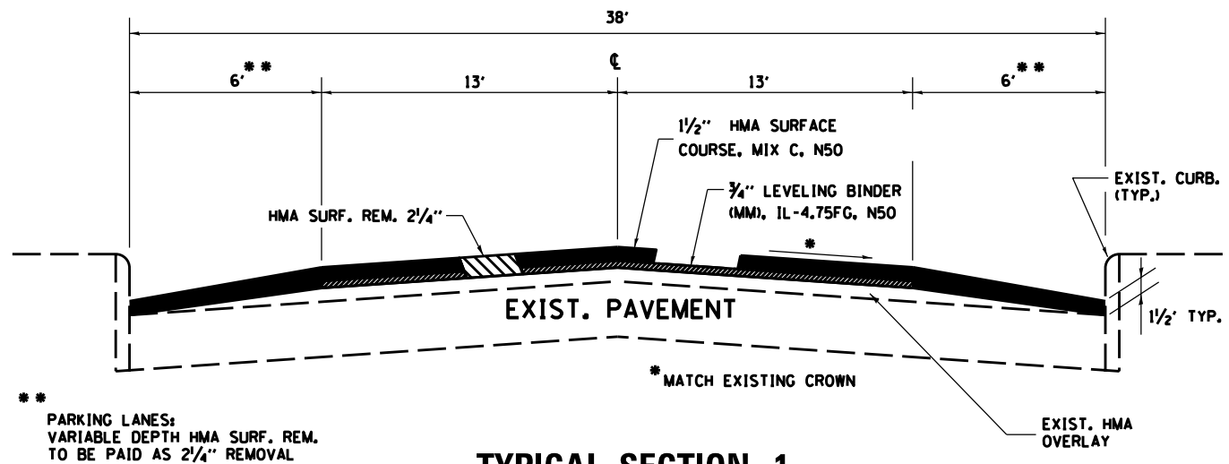
TYPICAL SECTION 1 PROPOSED U.S. ROUTE 45 (OAK ST.) STA. 2325+08 TO 2336+58
