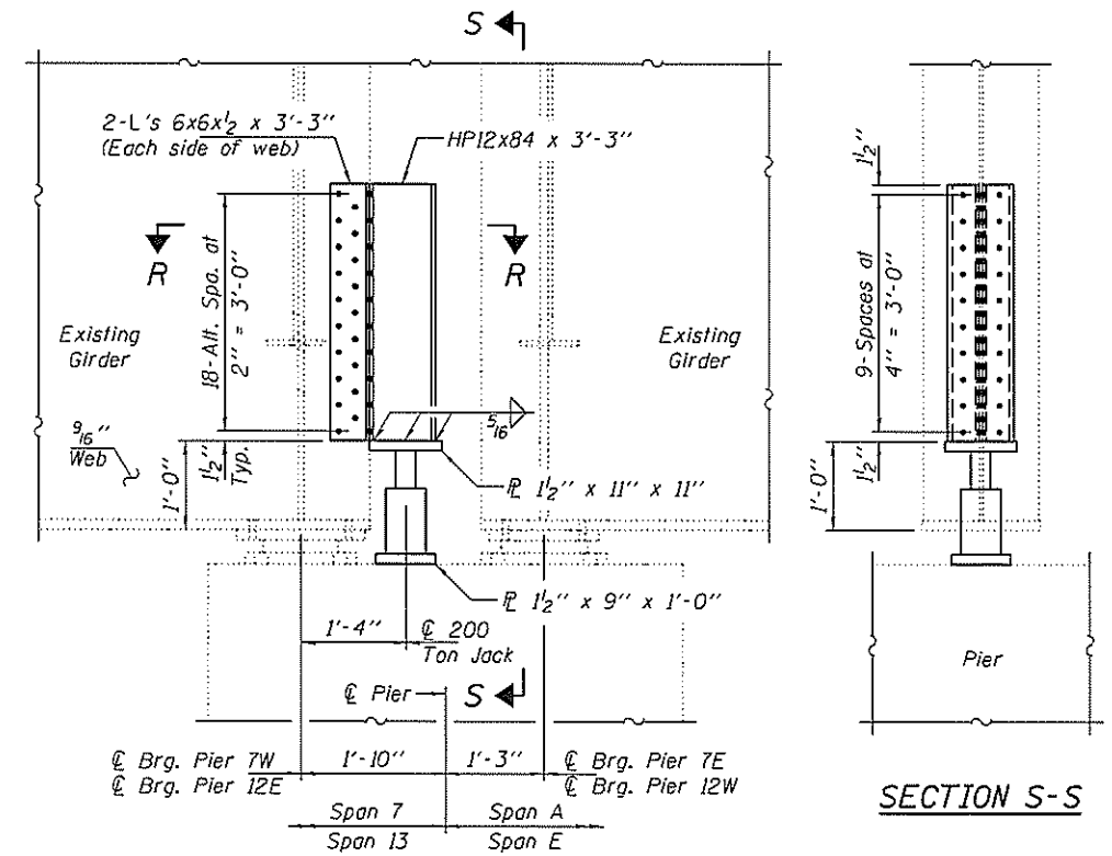
JACKING DETAIL FOR BEARING REPLACEMENT AT PIERS 7 & 12
