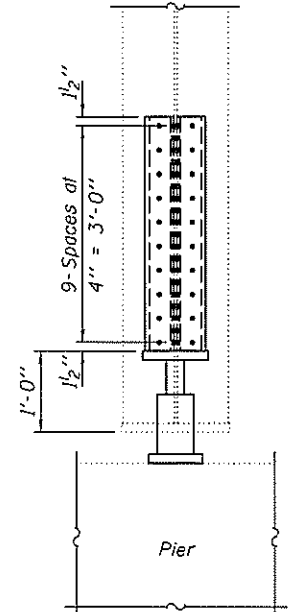
SECTION S-S
